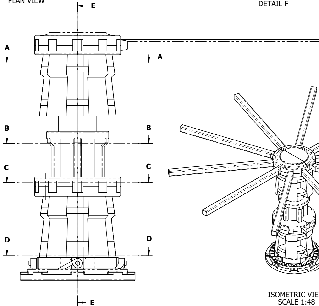
PLAN VIEW
